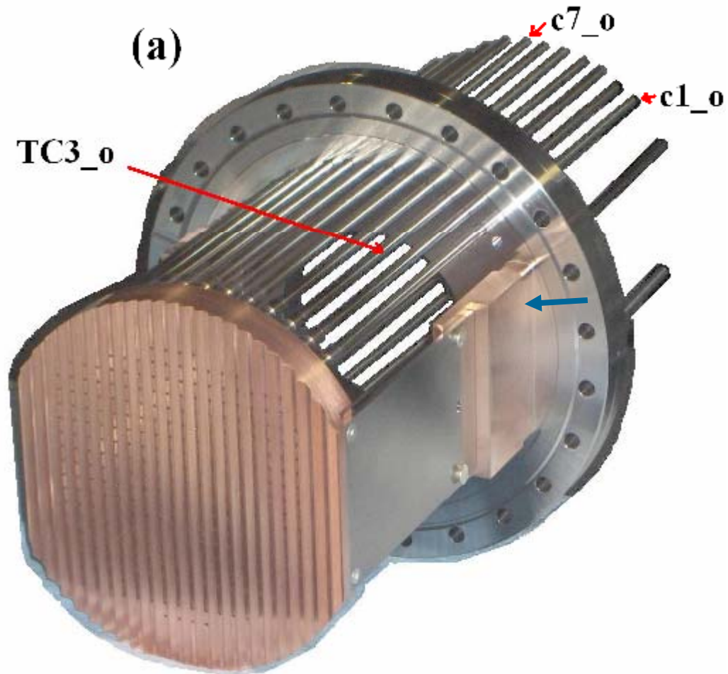
(a): Beam dump/calorimeter, with marks at some channels and thermocouple (TC) reserved positions; (c) with a cross for viewport and multipin feedthroughs assembly
