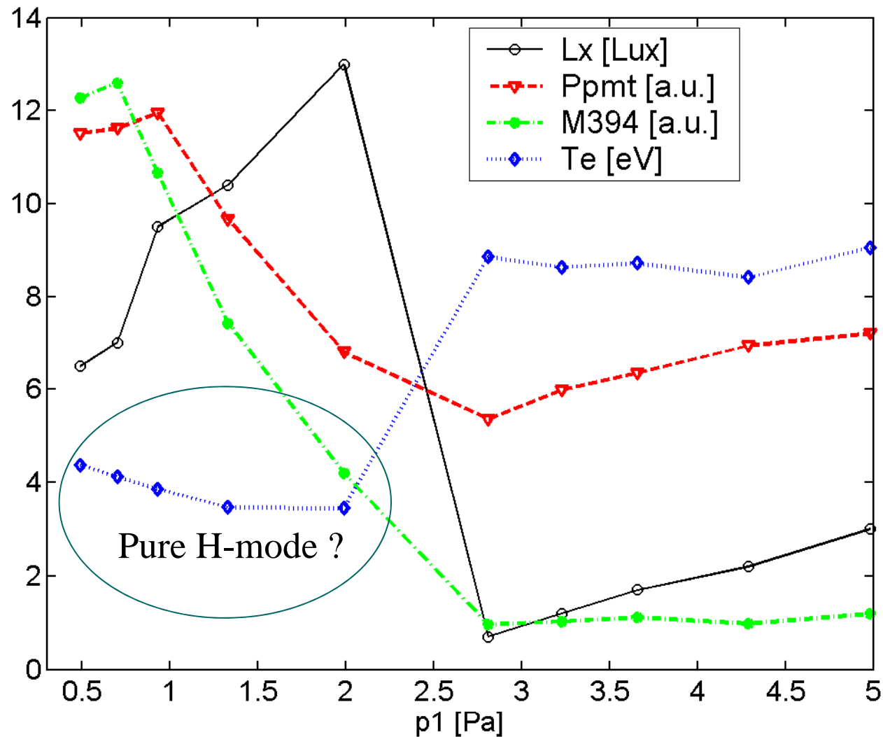
Figure : Plasma luminosity L_x vs source pressure p_1 (air) at constant net(*) rf power P = P_f - P_r = 0.47 \text{ kW} ; also shown P_{pmt} (1 a.u. = 10 mW) and M_{394} (1 a.u. = 10^{17} ph/s/m 2 ) and T_e ; typical error +/- 10 %
