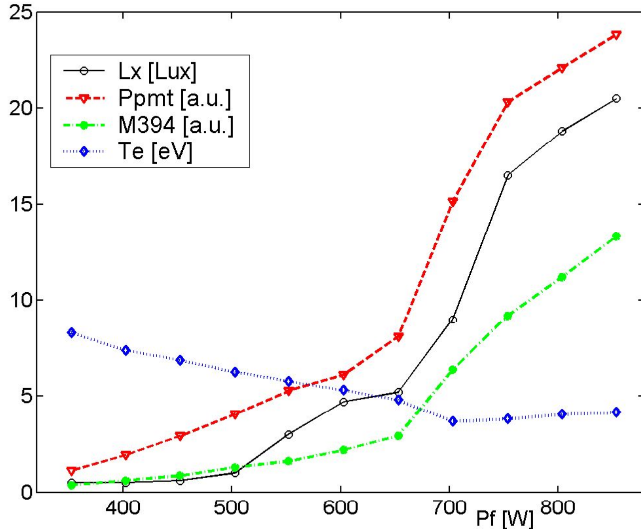
Figure : Plasma luminosity L_x vs forward rf power P_f at p_1 = 0.9 Pa; also shown P_{pmt} (1 a.u. = 10 mW) and M_{394} (1 a.u. = 10^{17} ph/s/m 2 ) and apparent electron temperature T_e ; typical error +/- 10 %
