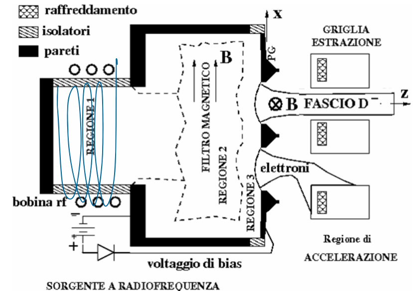
Figure: scheme of an rf driven negative ion source; region 3 (sheath) thickness exaggerated for visibility
